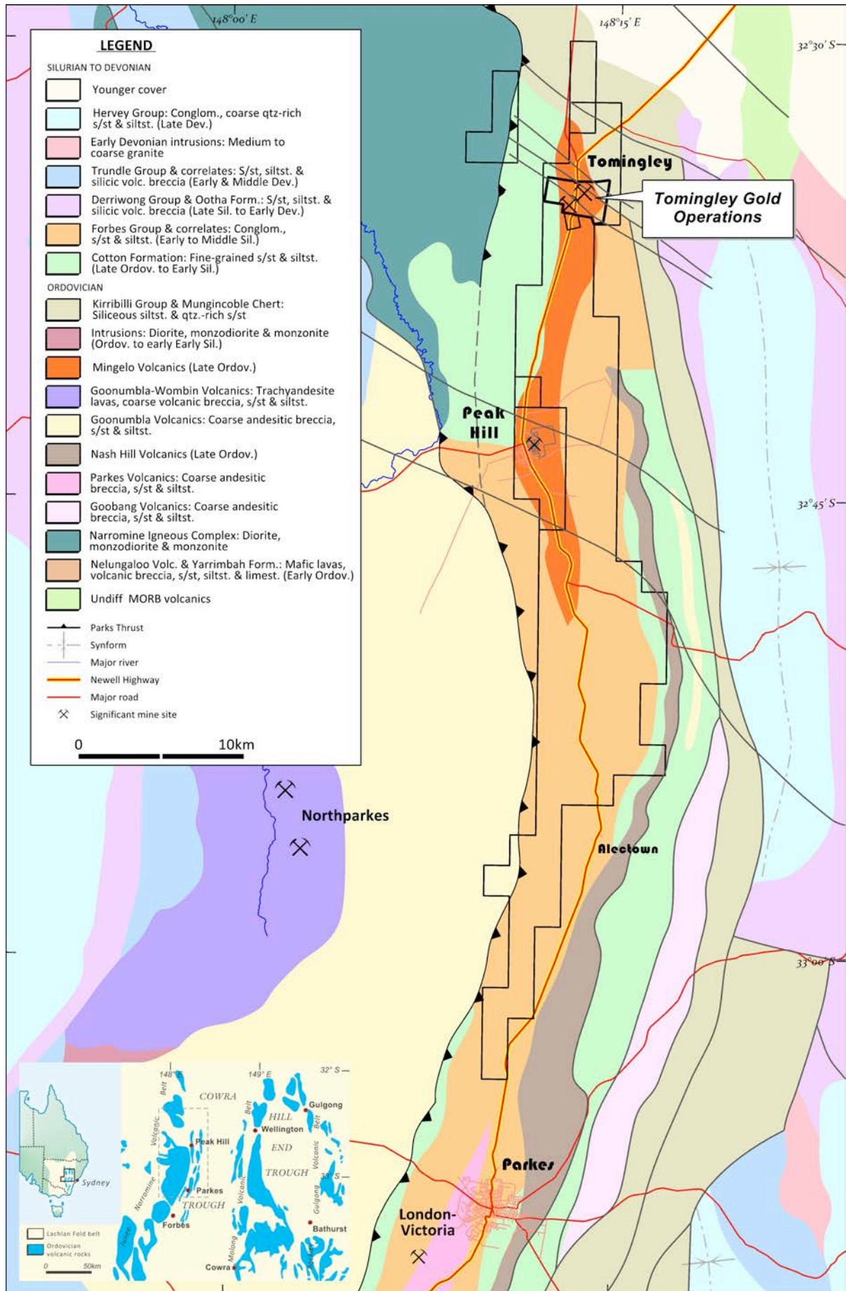
Figure 1: Regional geological setting
