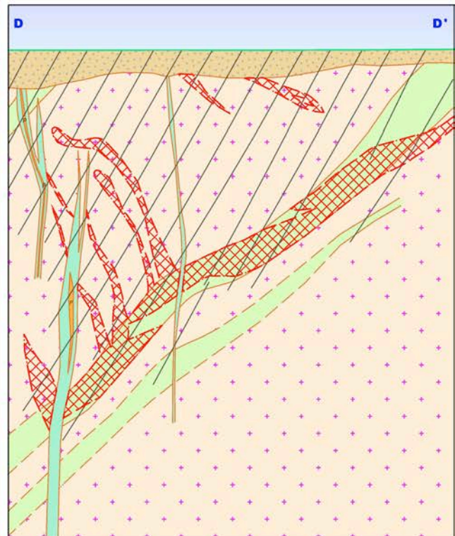
Figure 3d: Caloma Two cross section 614890mE MGA
