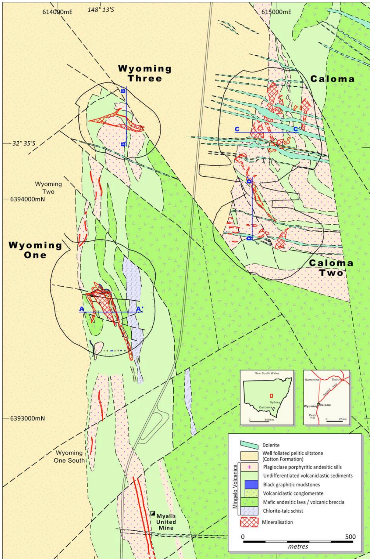
Figure 2: Mine site geology with pit shell outlines
